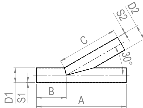
Stainless steel branch pipes 30°
